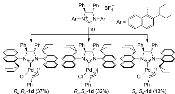
Scheme 2. Synthesis of 1d a
